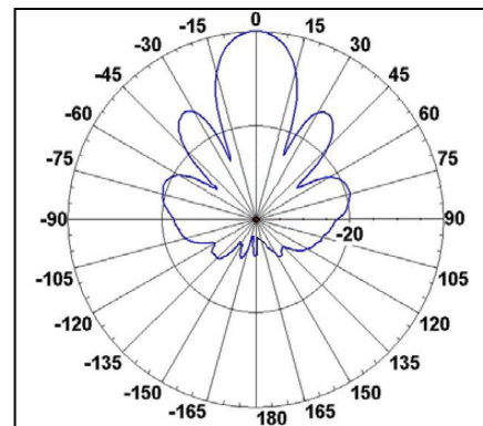
Horizontal Radiation pattern
