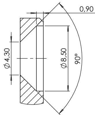
DETAIL B (QTY 8) SCALE 5 : 1
