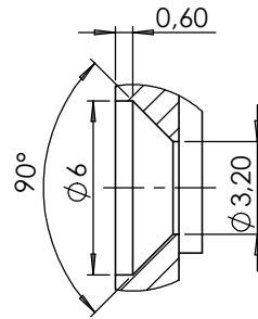
DETAIL C (QTY 6) SCALE 5 : 1
